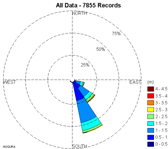
NGQURA Wave Height (Hmo) vs Wave Direction 2011-03-05 to 2014-02-28
