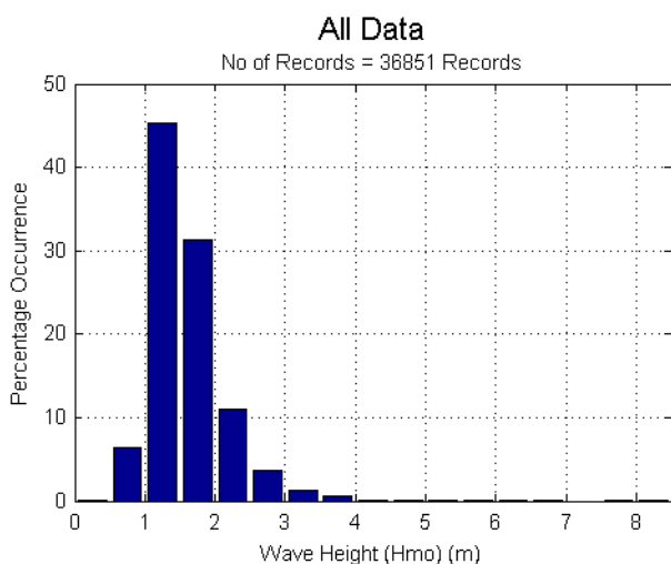
RICHARDS BAY Histogram of Wave Height (Hmo) 2000-03-01 to 2014-02-28
