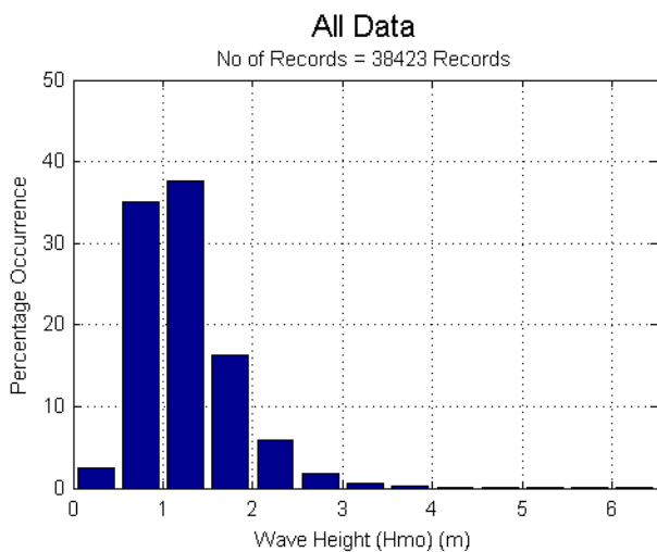
SALDANHA BAY Histogram of Wave Height (Hmo) 2000-03-01 to 2014-02-28
