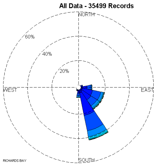
RICHARDS BAY Wave Height (Hmo) vs Wave Direction 2000-03-01 to 2014-02-28
